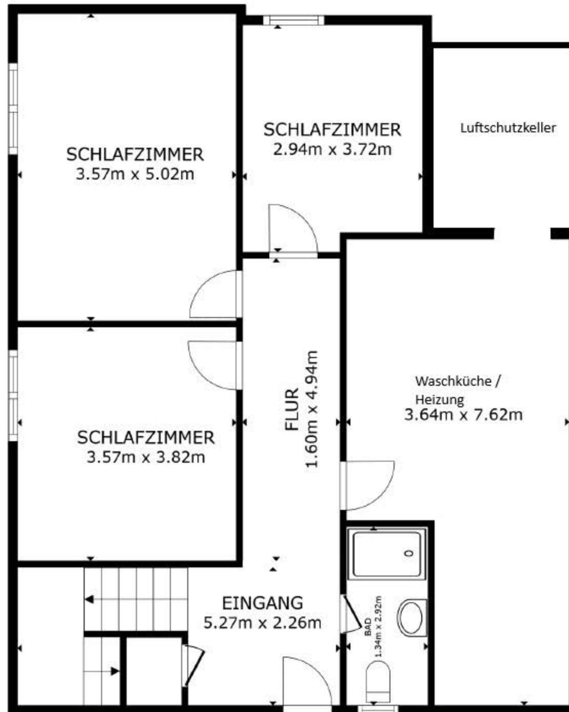
FLOOR PLAN
