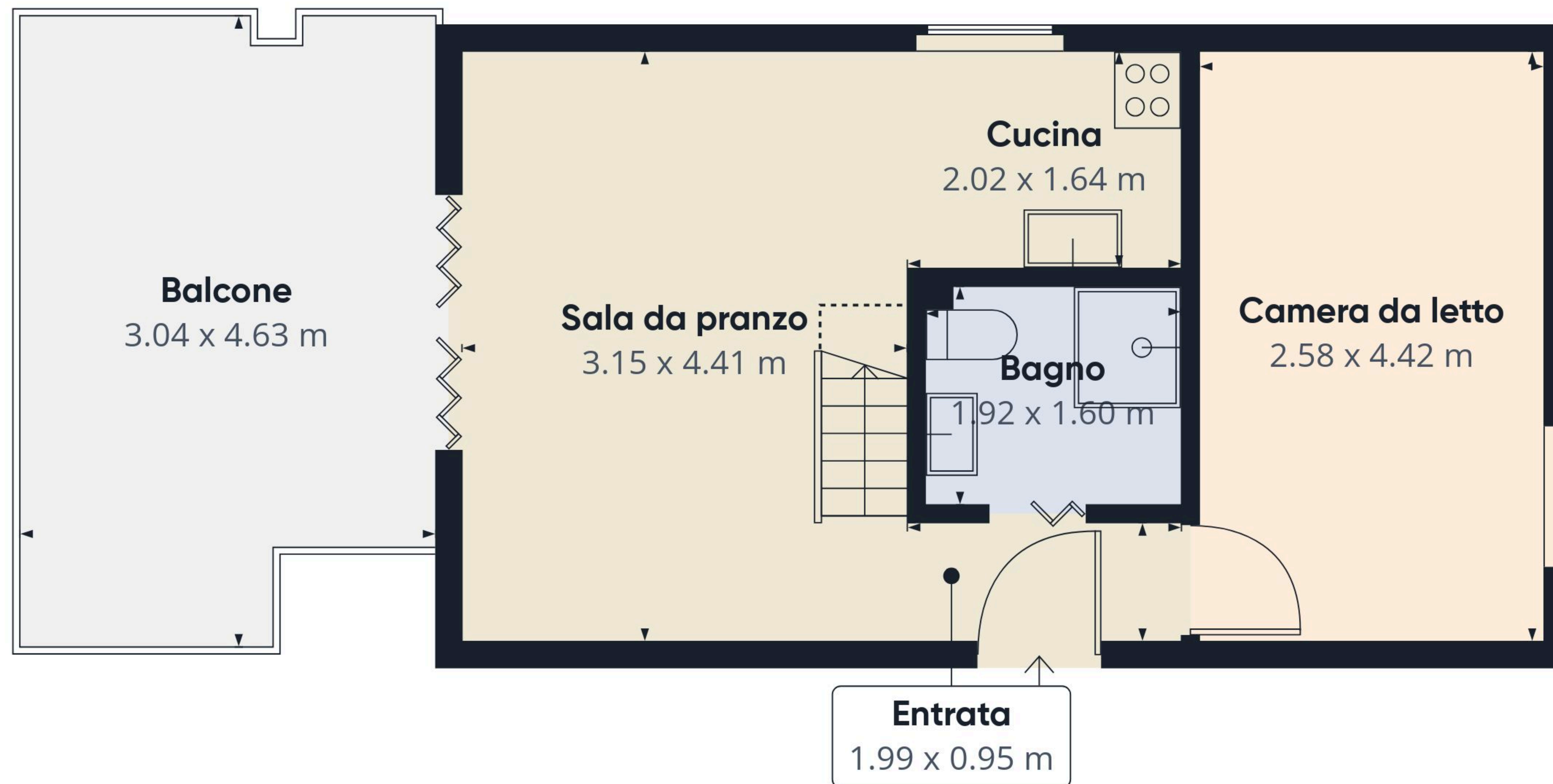
Ground Floor
